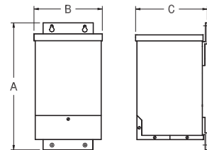
Outline Drawing 3 Wall Mount - Encapsulated - NEMA Type 3R
